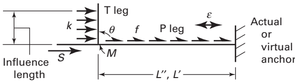
Fig. VII-3.3.2-2 Element Category B, Branch Pipe Joining the P Leg
