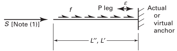
Fig. VII-3.3.2-4 Element Category D, Straight Pipe
