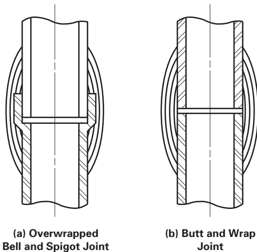
Fig. N-127.8.1(B) Thermosetting Resin Joints
