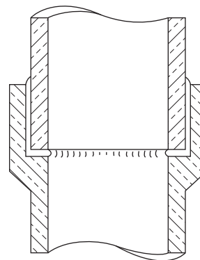
Fig. N-127.7.1(B) Solvent-Cemented Joint
