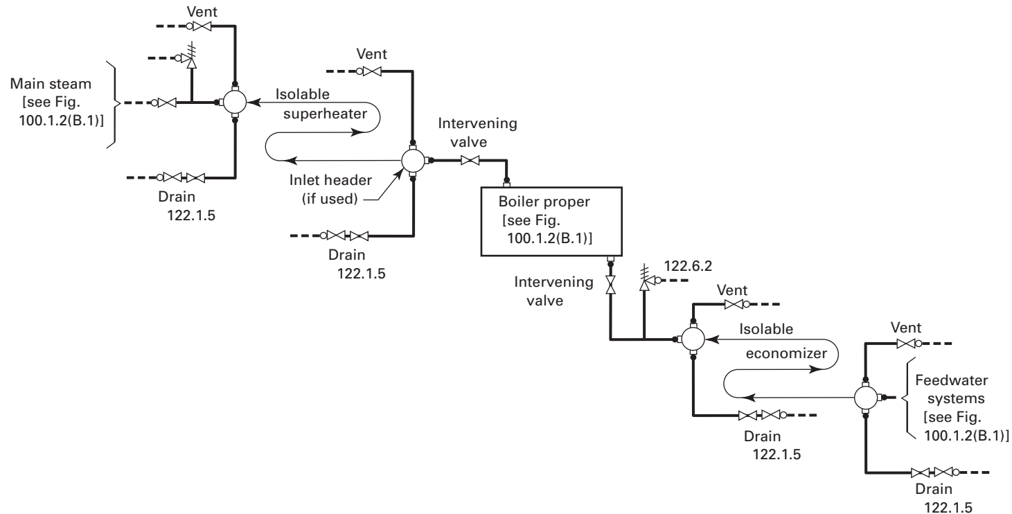
(16) Fig. 100.1.2(B.2) Code Jurisdictional Limits for Piping — Isolable Economizers Located in Feedwater Piping and Isolable Superheaters in Main Steam Piping (Boiler Pressure Relief Valves, Blowoff, and Miscellaneous Piping for Boiler Proper Not Shown for Clarity)
